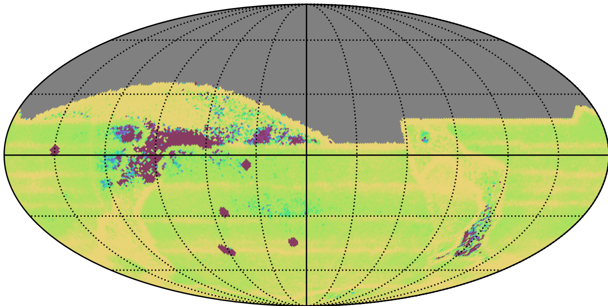
extra_ss_neo3_v3.4_10yrs All sky: Median Intra-Night Gap
