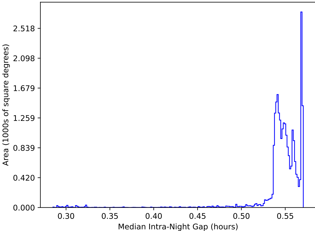
extra_ss_neo3_v3.4_10yrs All sky: Median Intra-Night Gap
