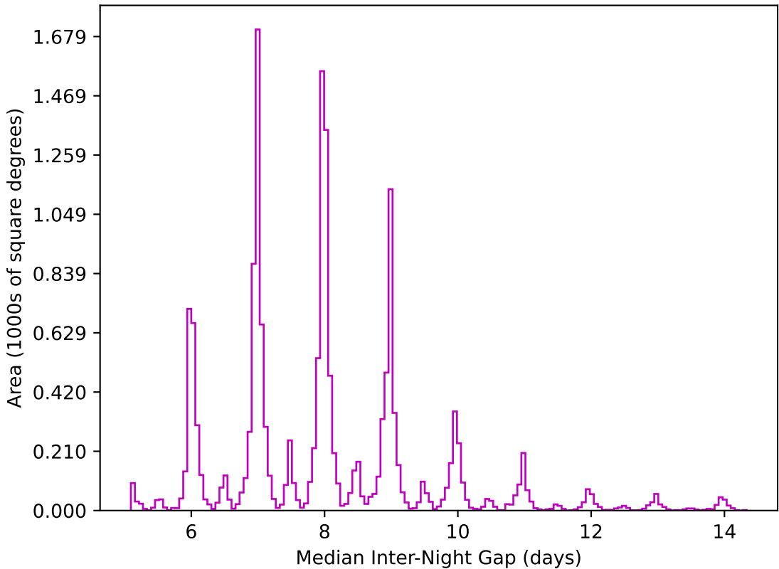
extra_ss_neo3_v3.4_10yrs WFD z band: Median Inter-Night Gap
