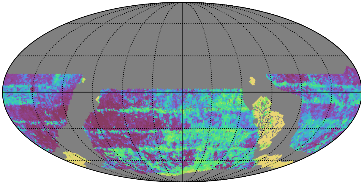
extra_ss_neo3_v3.4_10yrs WFD y band: Median Inter-Night Gap
