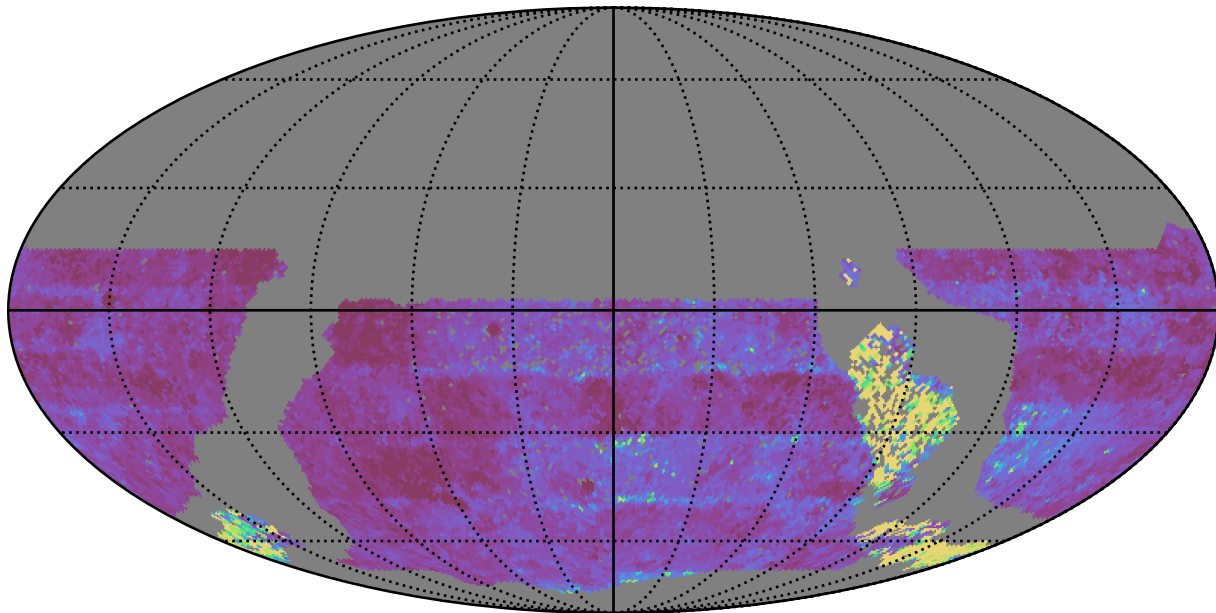
extra_ss_neo3_v3.4_10yrs WFD u band: Median Inter-Night Gap
