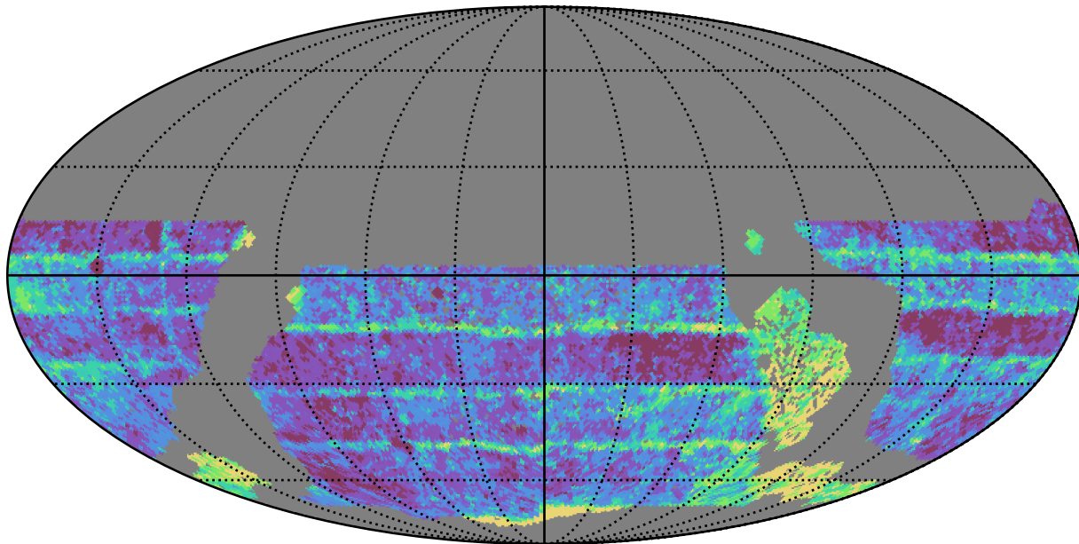
extra_ss_neo3_v3.4_10yrs WFD i band: Median Inter-Night Gap
