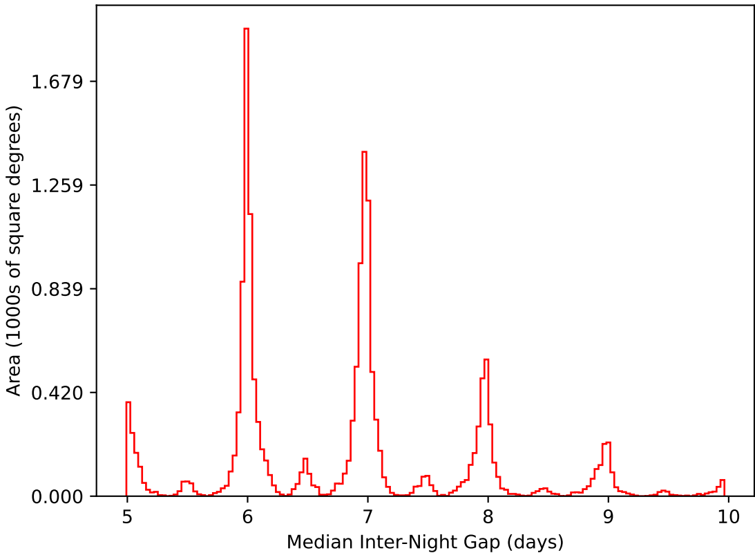
extra_ss_neo3_v3.4_10yrs WFD i band: Median Inter-Night Gap
