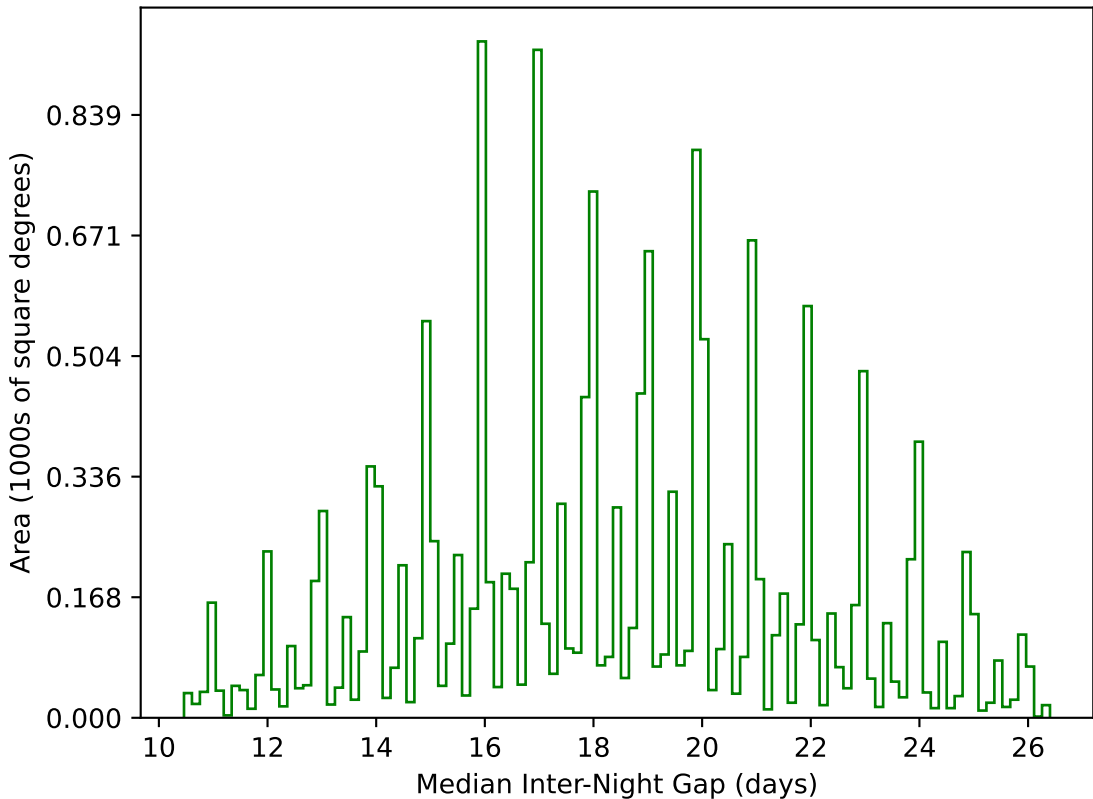
extra_ss_neo3_v3.4_10yrs WFD g band: Median Inter-Night Gap
