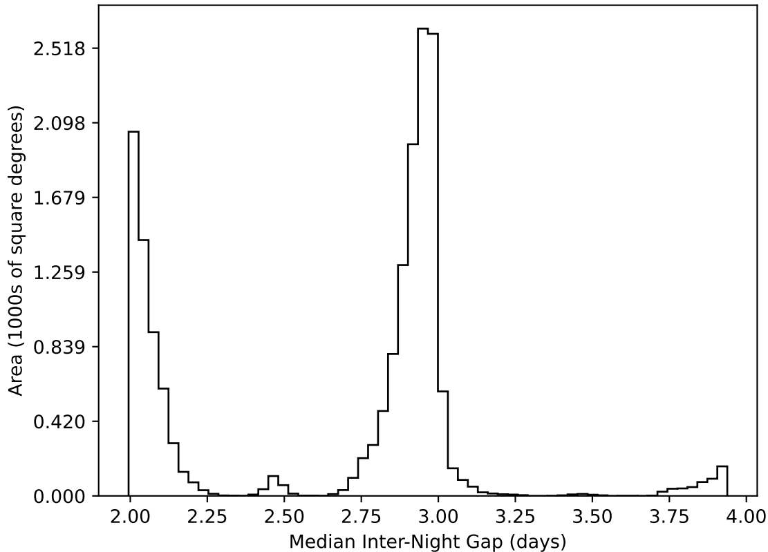
extra_ss_neo3_v3.4_10yrs WFD all bands: Median Inter-Night Gap
