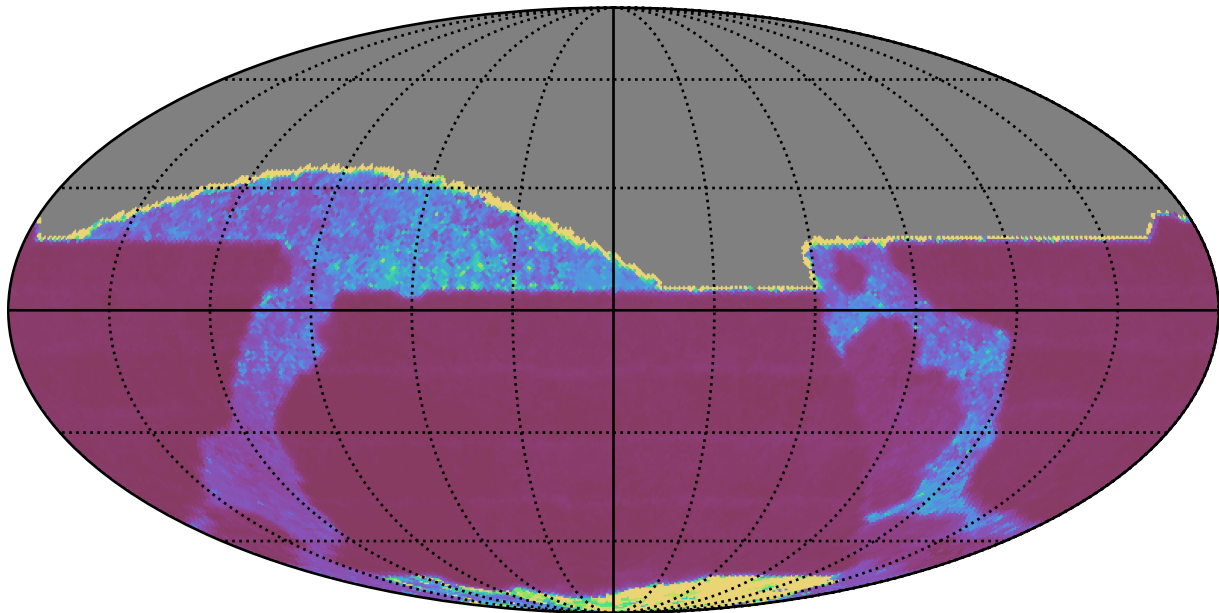
extra_ss_neo3_v3.4_10yrs All sky z band: Median Inter-Night Gap
