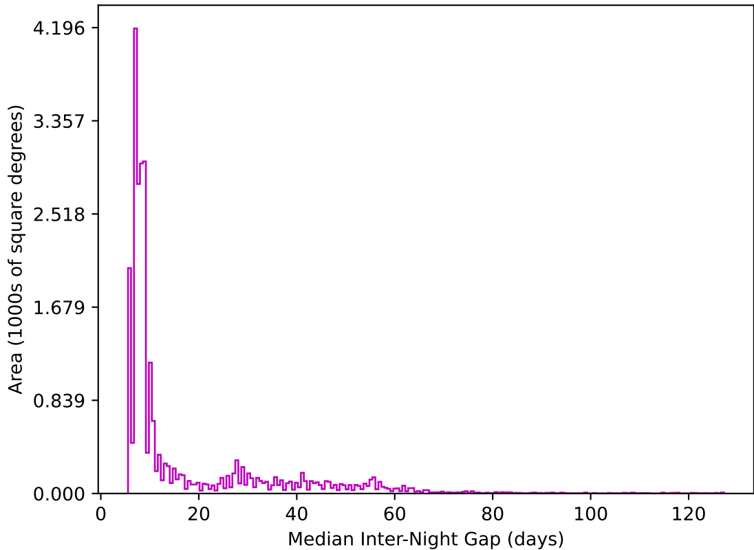
extra_ss_neo3_v3.4_10yrs All sky z band: Median Inter-Night Gap
