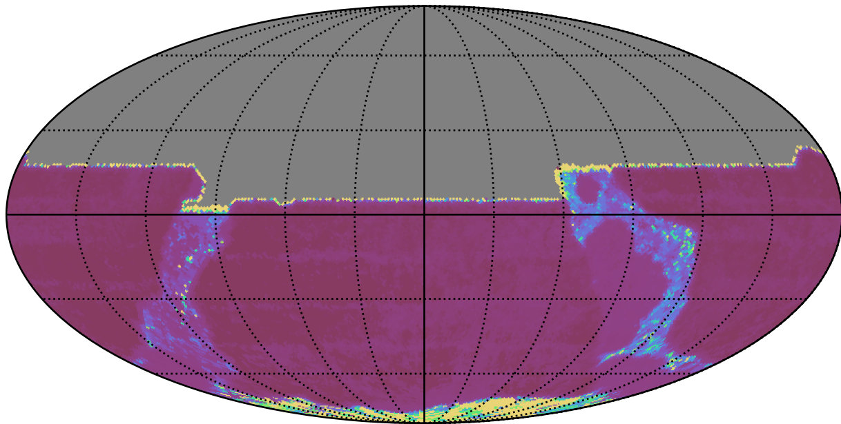
extra_ss_neo3_v3.4_10yrs All sky y band: Median Inter-Night Gap
