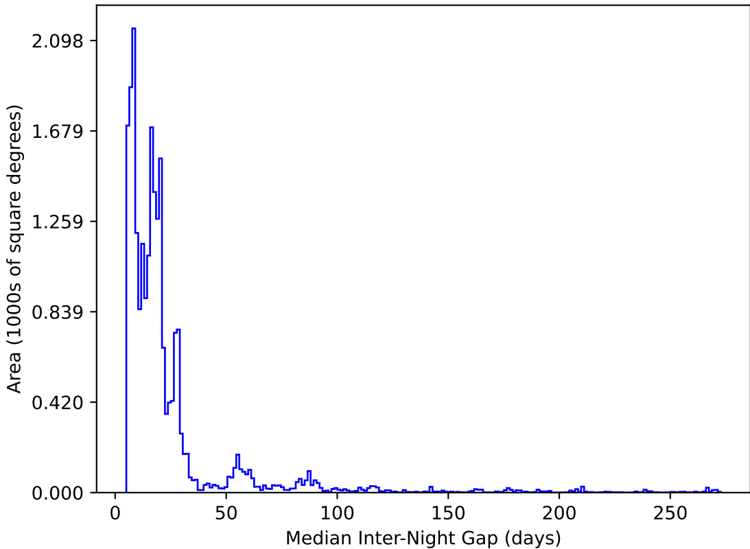
extra_ss_neo3_v3.4_10yrs All sky y band: Median Inter-Night Gap
