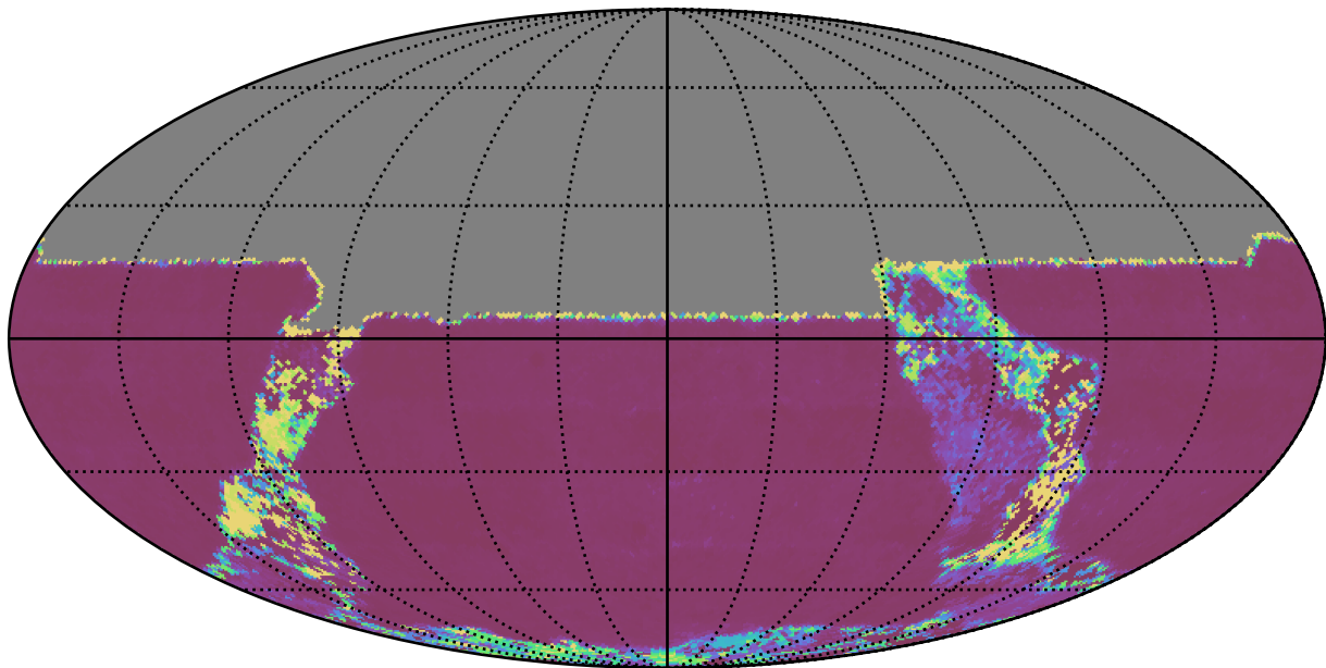
extra_ss_neo3_v3.4_10yrs All sky u band: Median Inter-Night Gap
