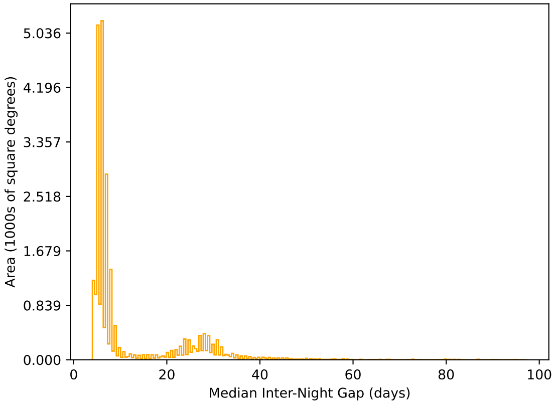
extra_ss_neo3_v3.4_10yrs All sky r band: Median Inter-Night Gap
