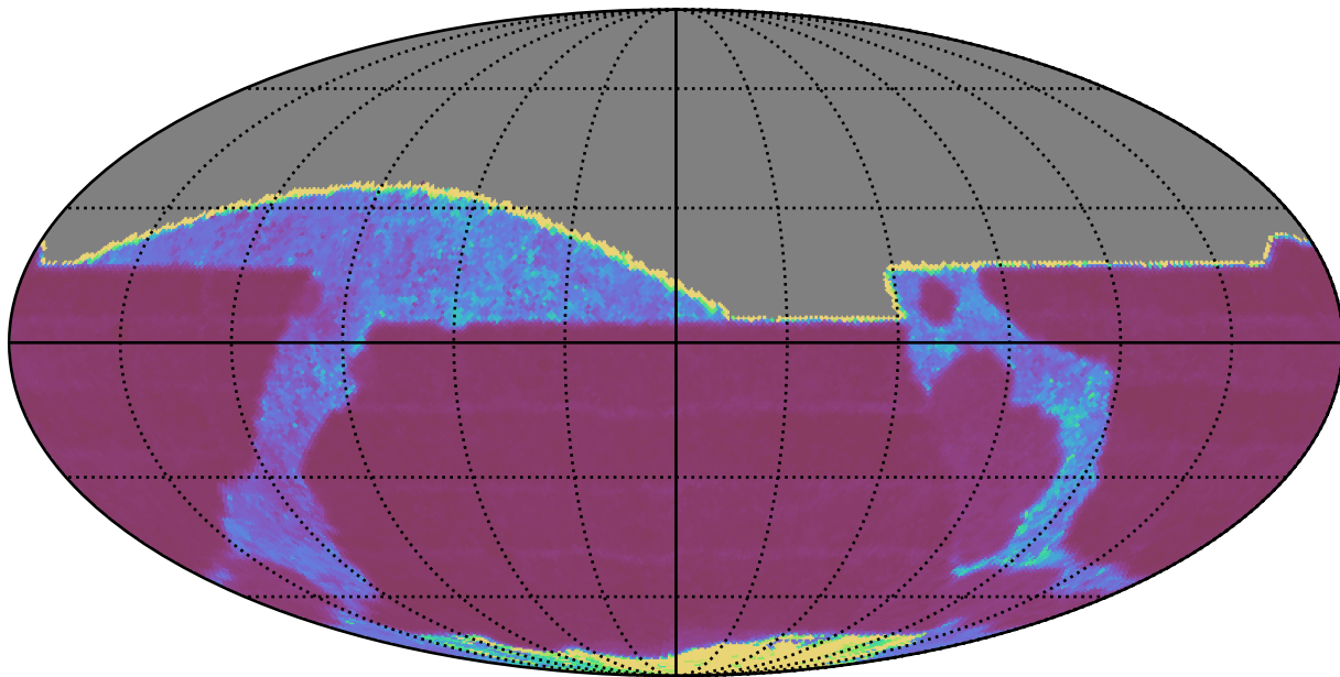
extra_ss_neo3_v3.4_10yrs All sky i band: Median Inter-Night Gap
