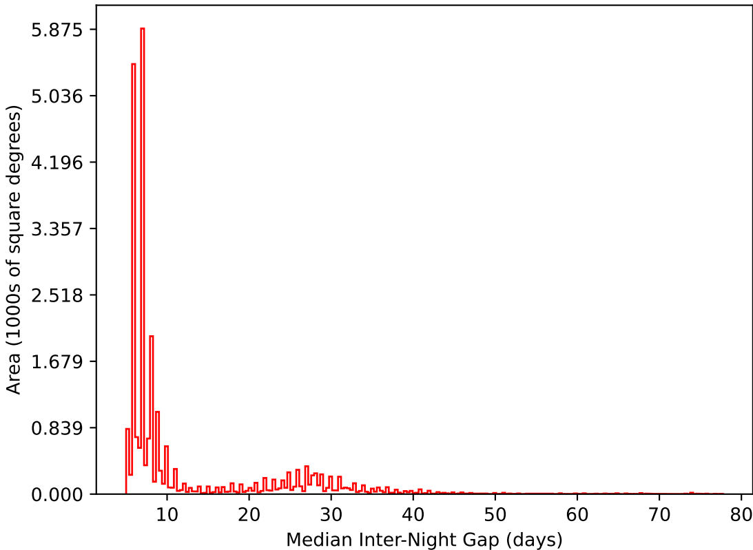
extra_ss_neo3_v3.4_10yrs All sky i band: Median Inter-Night Gap
