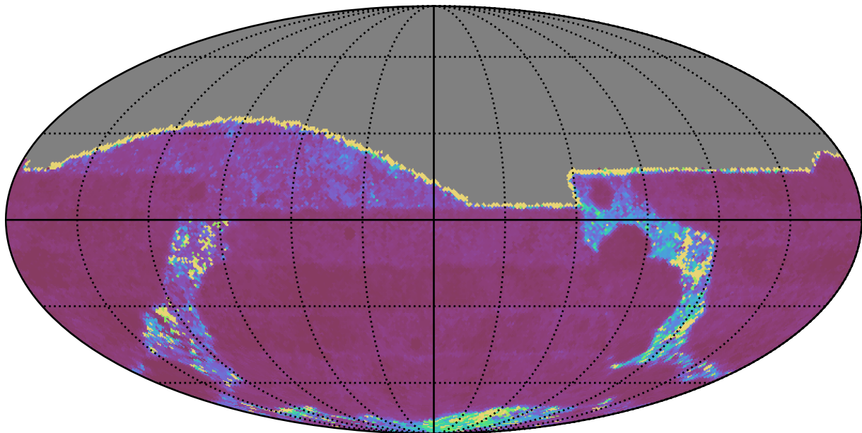
extra_ss_neo3_v3.4_10yrs All sky g band: Median Inter-Night Gap
