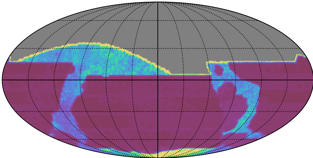
extra_ss_neo3_v3.4_10yrs All sky all bands: Median Inter-Night Gap
