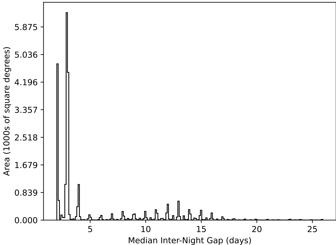
extra_ss_neo3_v3.4_10yrs All sky all bands: Median Inter-Night Gap
