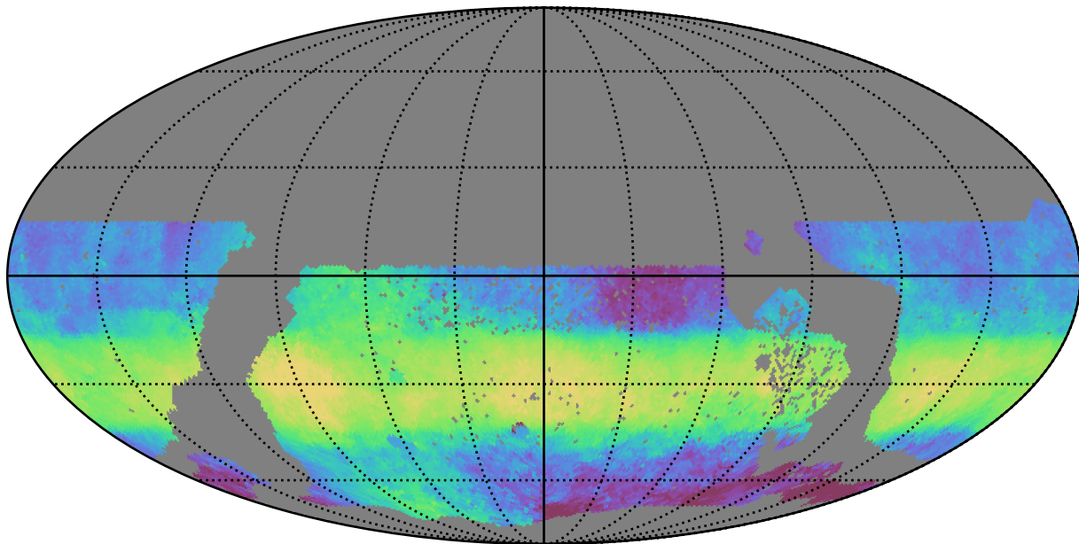
extra_ss_neo3_v3.4_10yrs WFD z band: Median HA
