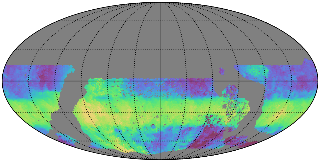
extra_ss_neo3_v3.4_10yrs WFD u band: Median HA
