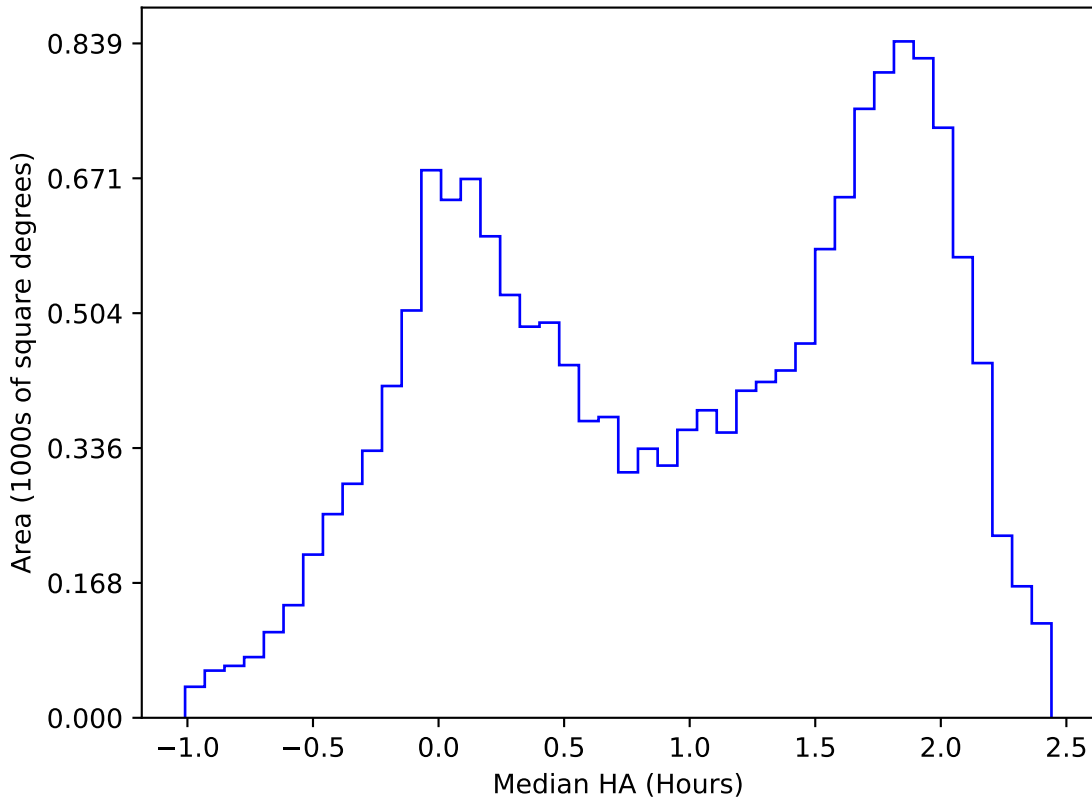
extra_ss_neo3_v3.4_10yrs WFD u band: Median HA
