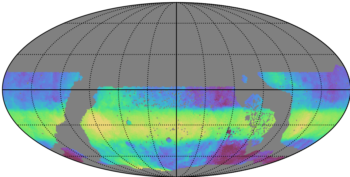
extra_ss_neo3_v3.4_10yrs WFD r band: Median HA
