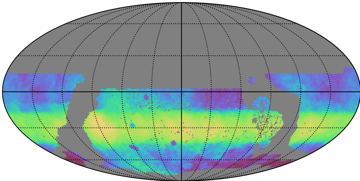
extra_ss_neo3_v3.4_10yrs WFD i band: Median HA
