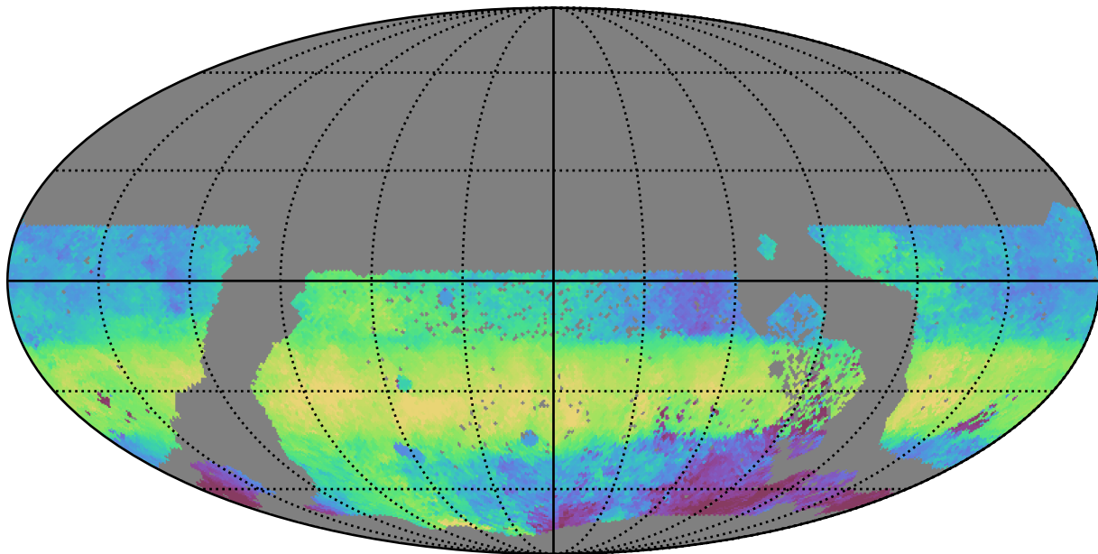
extra_ss_neo3_v3.4_10yrs WFD g band: Median HA
