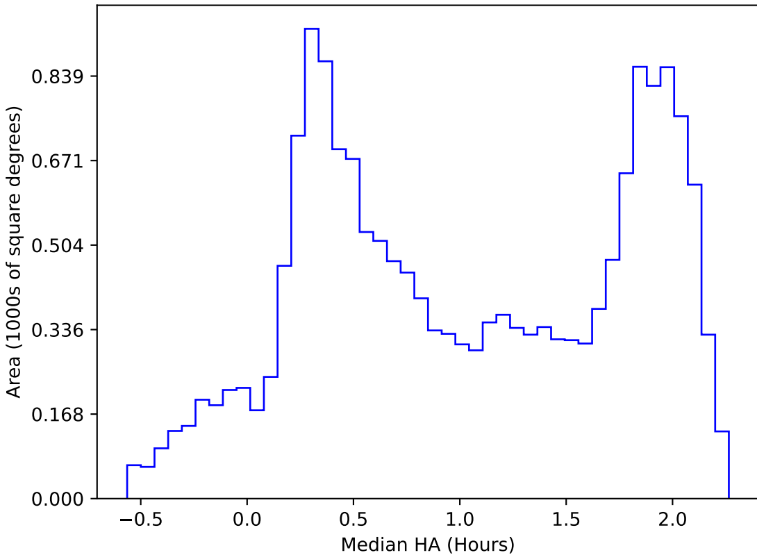
extra_ss_neo3_v3.4_10yrs WFD all bands: Median HA
