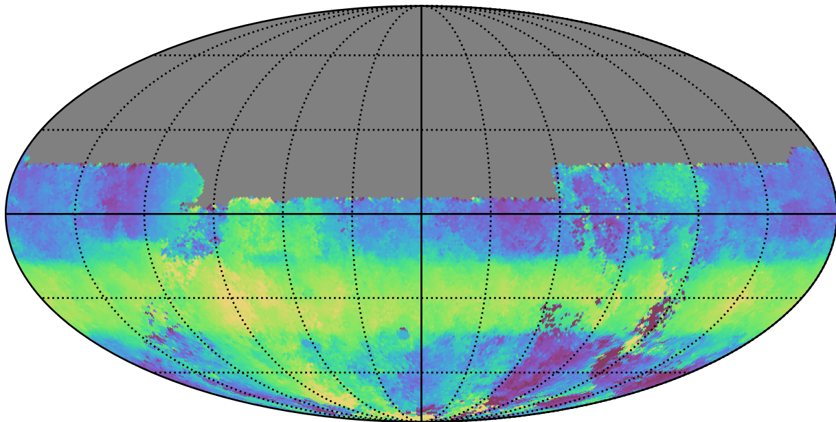
extra_ss_neo3_v3.4_10yrs All sky u band: Median HA
