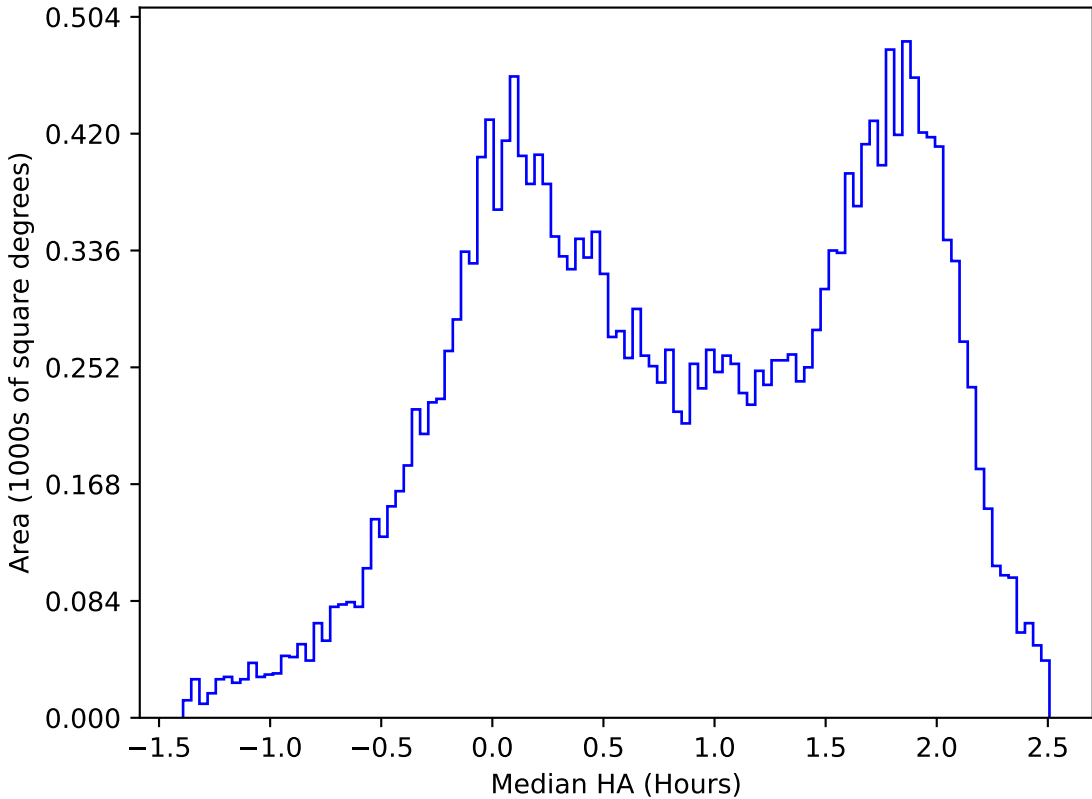
extra_ss_neo3_v3.4_10yrs All sky u band: Median HA
