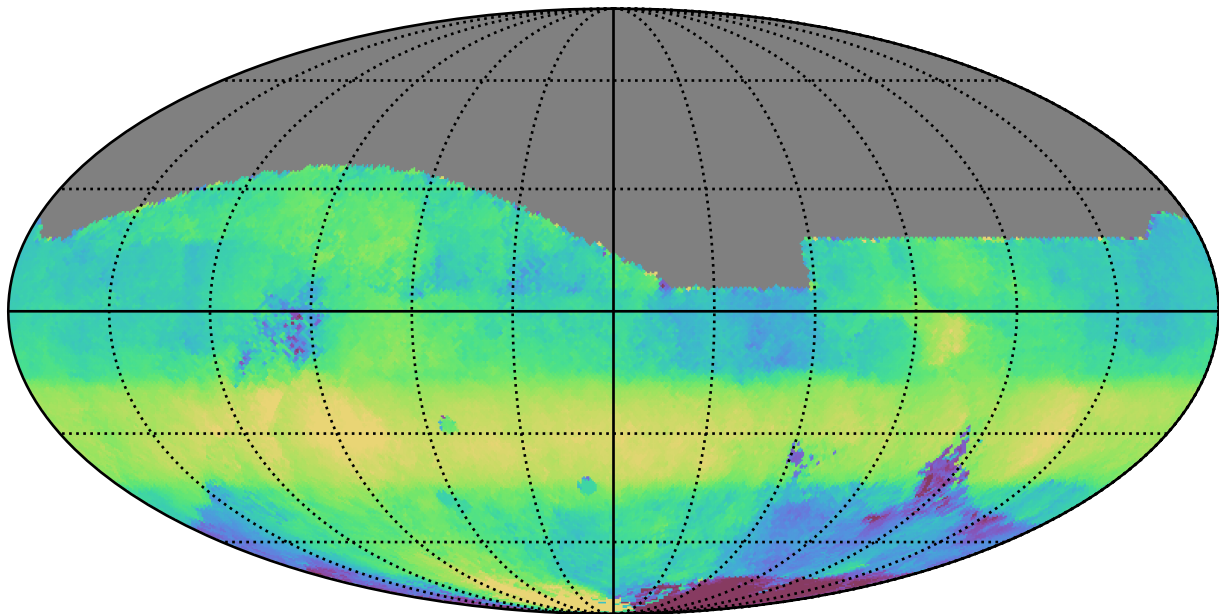
extra_ss_neo3_v3.4_10yrs All sky r band: Median HA
