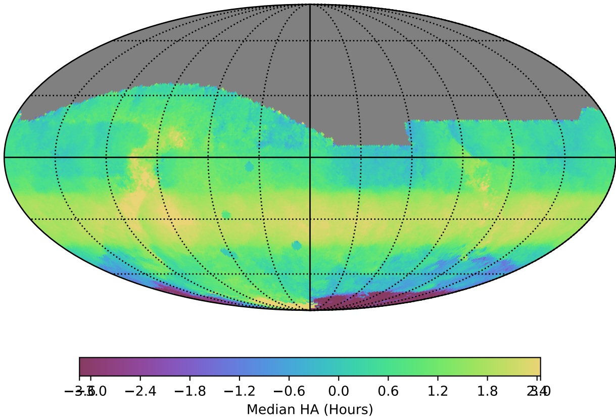
extra_ss_neo3_v3.4_10yrs All sky i band: Median HA
