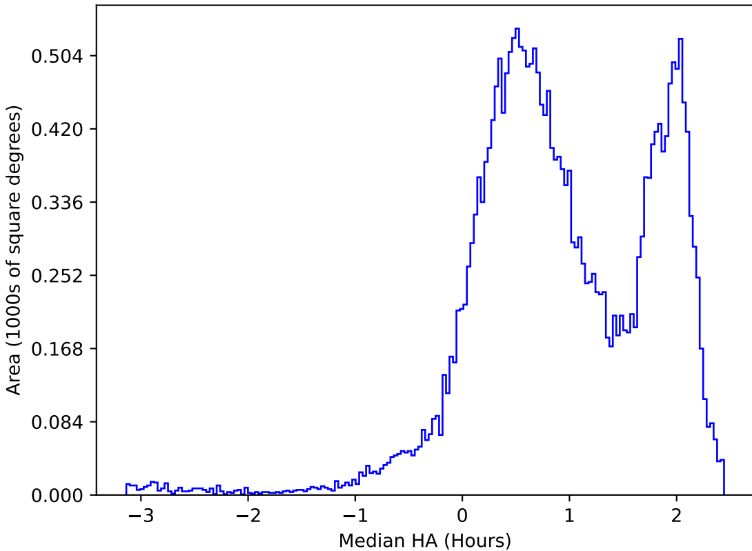
extra_ss_neo3_v3.4_10yrs All sky i band: Median HA
