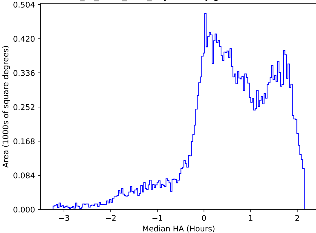
extra_ss_neo3_v3.4_10yrs All sky g band: Median HA
