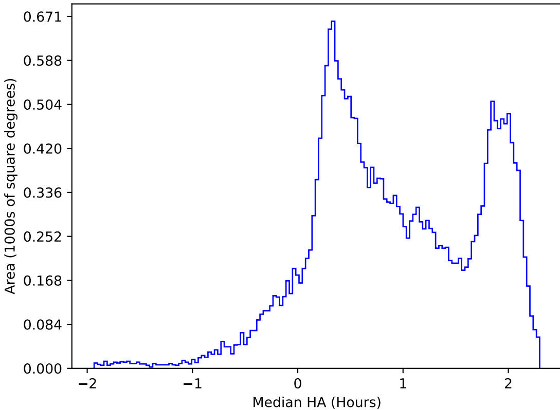
extra_ss_neo3_v3.4_10yrs All sky all bands: Median HA
