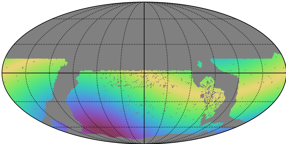
extra_ss_neo3_v3.4_10yrs WFD all bands: Max solarElong
