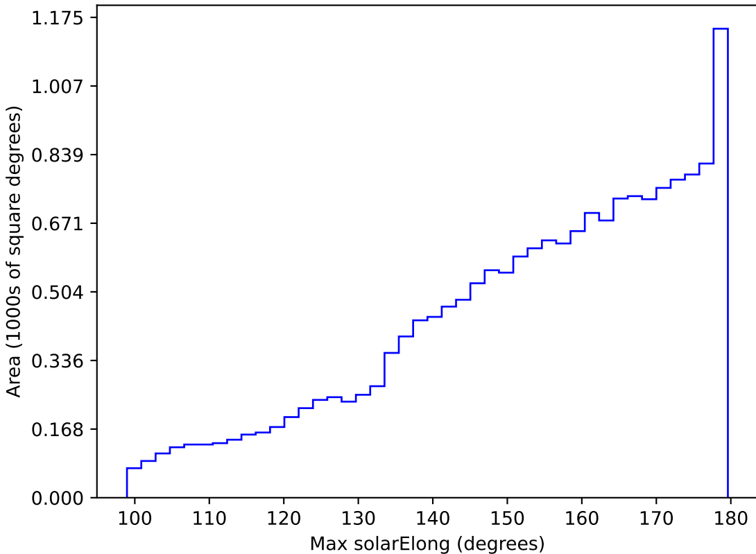
extra_ss_neo3_v3.4_10yrs WFD all bands: Max solarElong
