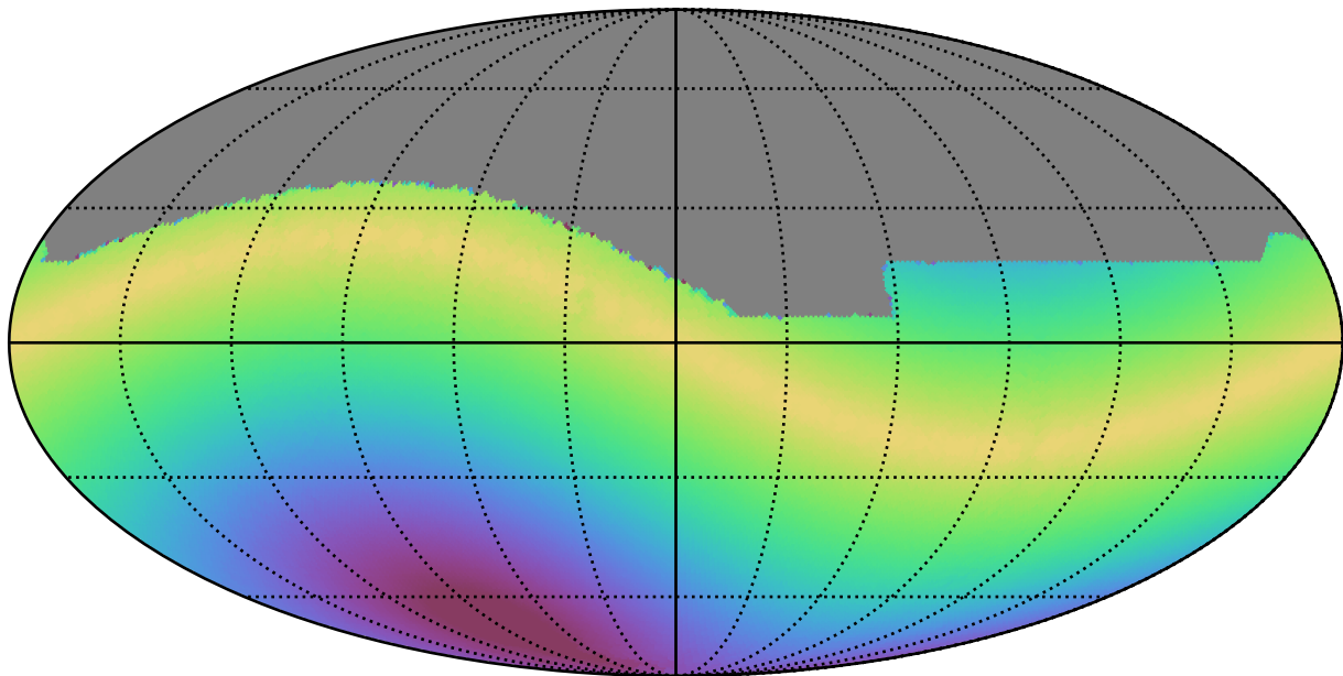
extra_ss_neo3_v3.4_10yrs All sky all bands: Max solarElong
