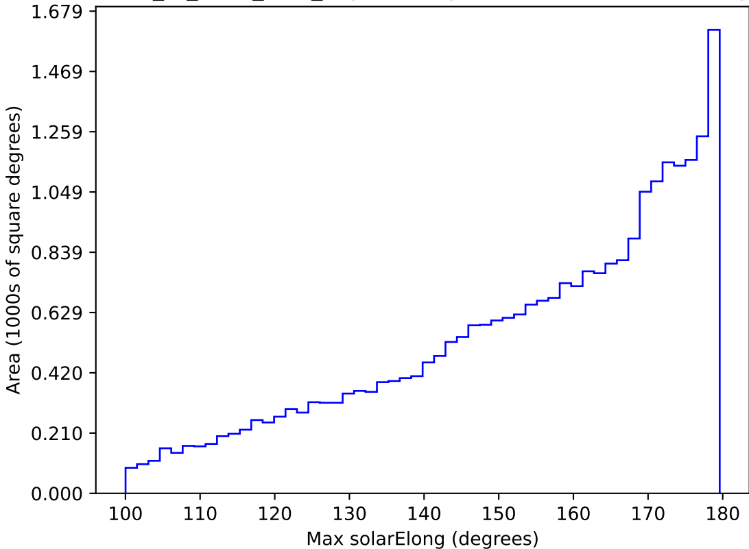
extra_ss_neo3_v3.4_10yrs All sky all bands: Max solarElong
