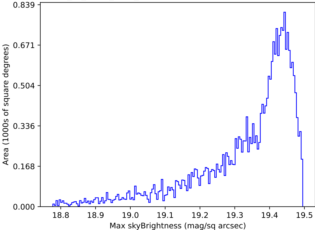
extra_ss_neo3_v3.4_10yrs Yr 1 z band: Max skyBrightness
