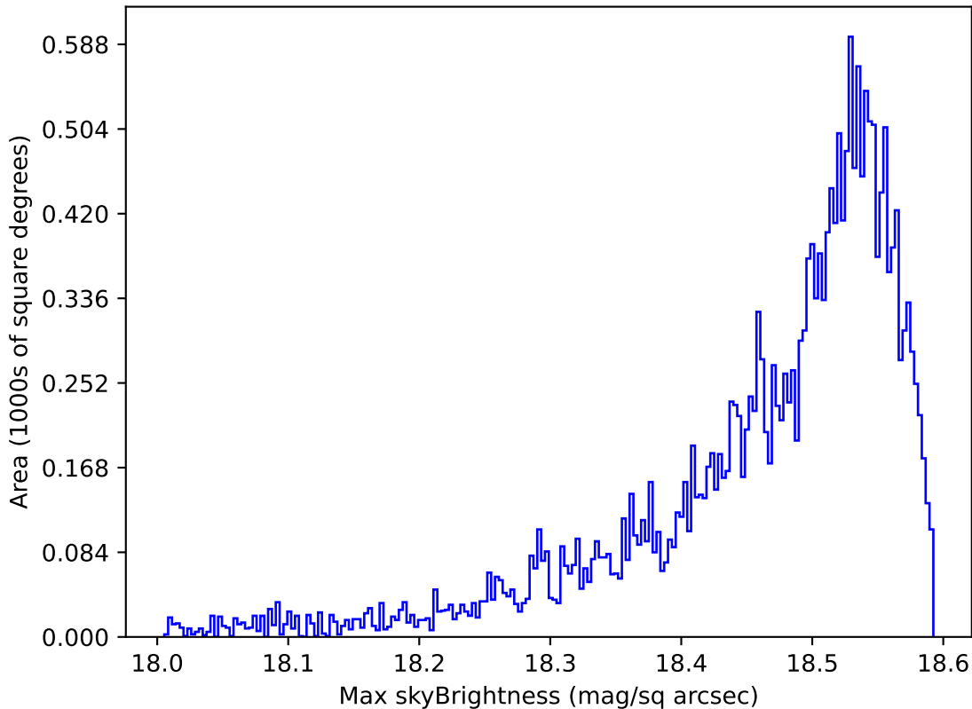
extra_ss_neo3_v3.4_10yrs Yr 1 y band: Max skyBrightness
