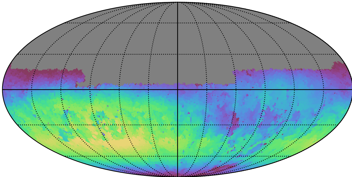
extra_ss_neo3_v3.4_10yrs Yr 1 u band: Max skyBrightness
