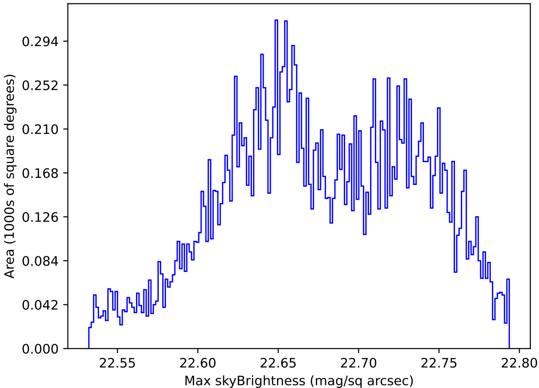
extra_ss_neo3_v3.4_10yrs Yr 1 u band: Max skyBrightness
