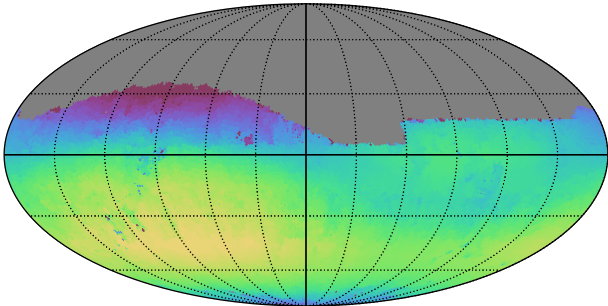
extra_ss_neo3_v3.4_10yrs Yr 1 r band: Max skyBrightness
