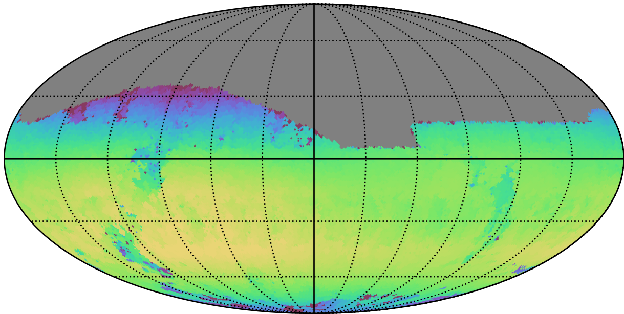
extra_ss_neo3_v3.4_10yrs Yr1 i band: Max skyBrightness
