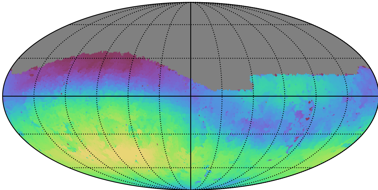
extra_ss_neo3_v3.4_10yrs Yr 1 g band: Max skyBrightness
