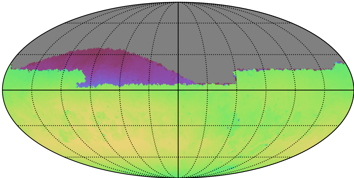
extra_ss_neo3_v3.4_10yrs Yr 1 all bands: Max skyBrightness
