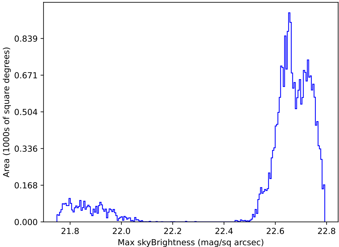
extra_ss_neo3_v3.4_10yrs Yr 1 all bands: Max skyBrightness
