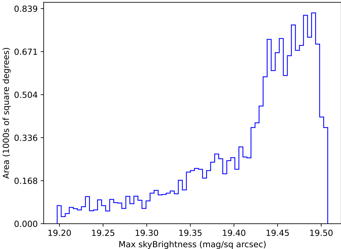
extra_ss_neo3_v3.4_10yrs WFD z band: Max skyBrightness
