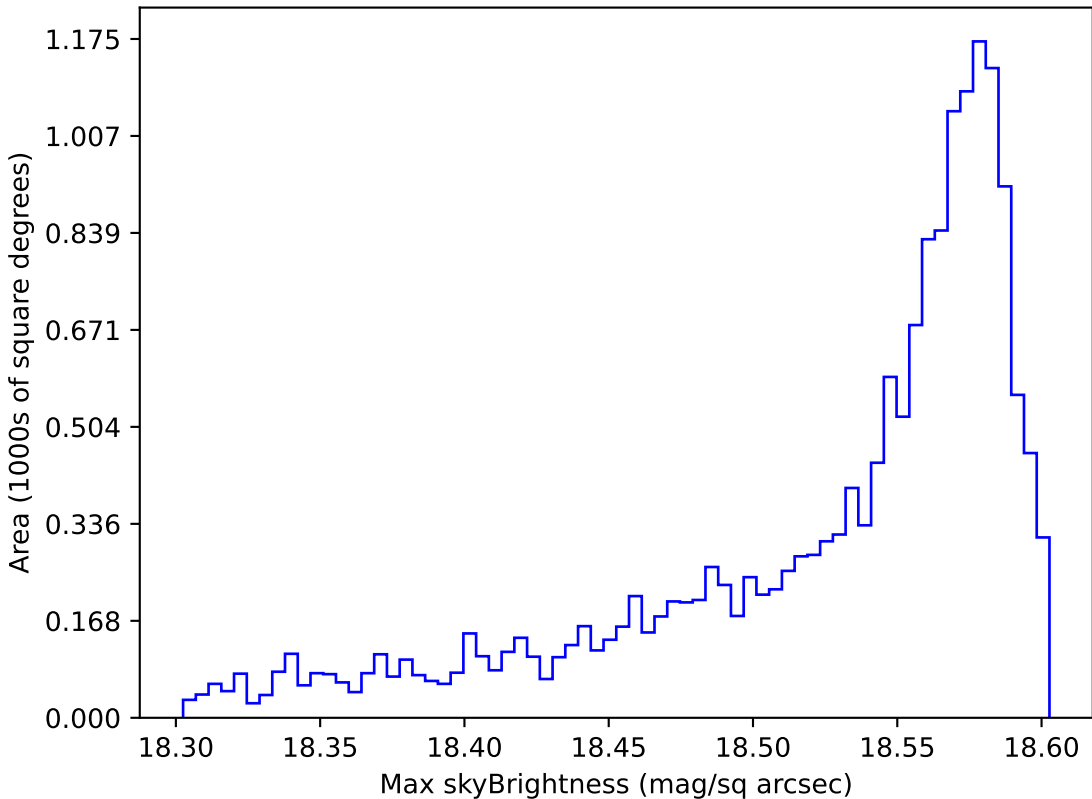
extra_ss_neo3_v3.4_10yrs WFD y band: Max skyBrightness
