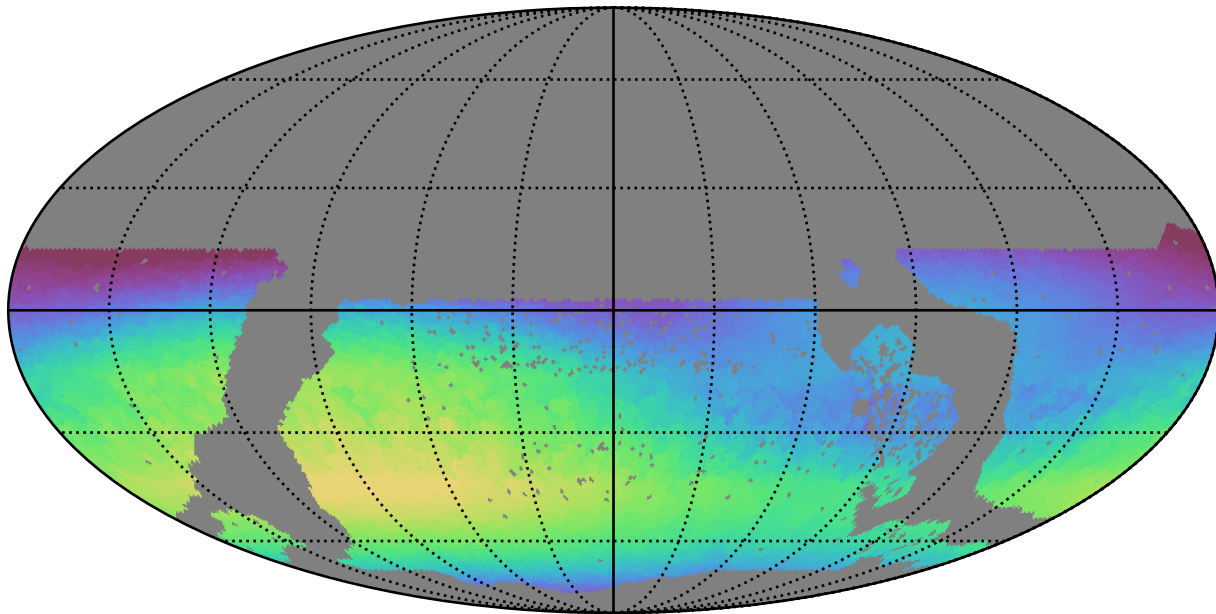
extra_ss_neo3_v3.4_10yrs WFD u band: Max skyBrightness
